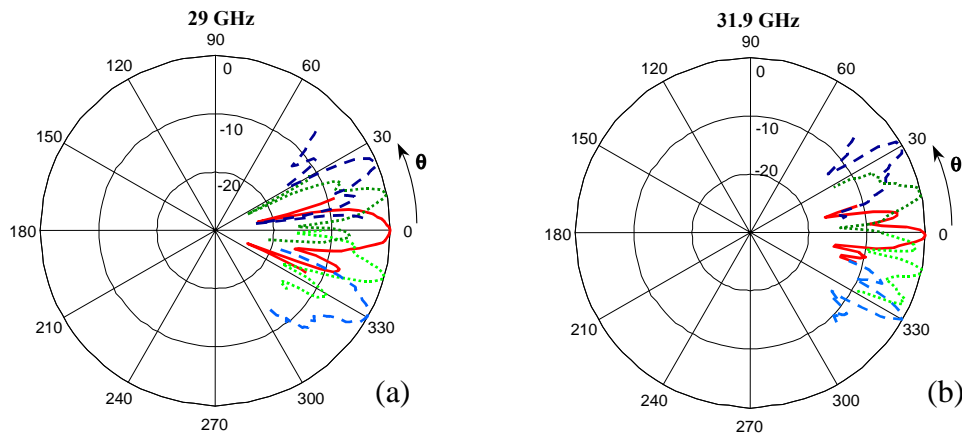
Fig. 4. Measured radiation patterns demonstrating the multibeam capabilities of a planar lens for (a) 29GHz, with the feed vertically polarized, and (b) 31.9 GHz, with the feed horizontally polarized. The plotted radiation pattern are generated by a feed positioned on axis (solid), at an angle \alpha=\pm 15^\circ (dotted) and at an angle \alpha=\pm 30^\circ (dashed)
