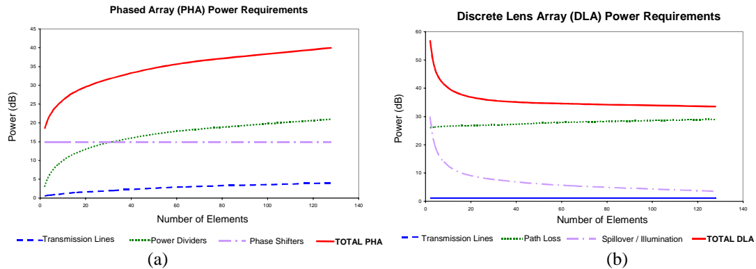
Fig. 2. Power requirements as a function of number of elements for (a) phased arrays (PHA) and (b) discrete planar lenses (DLA). Together with the total amount of power required to give equivalent performance, individual contributions to both systems are also illustrated.
