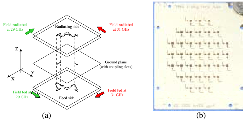
Fig. 3. (a) An exploded three-dimensional drawing of one element of the planar lens. The coupling between the transmission lines on the two sides of the lens is accomplished with slots in the common ground plane. (b) Photograph of the radiating side of the planar lens compared with a US quarter coin. Two different frequencies (29 and 31 GHz in the prototype) are radiated using two different linear polarizations.
