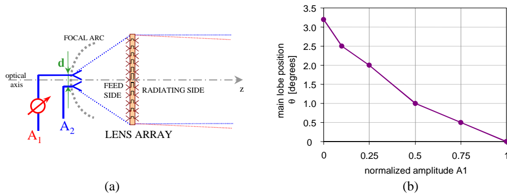
Fig. 5. (a) Schematic of the amplitude-controlled small scan angle configuration used in the simulations. (b) Simulation results showing the small angle scanning of the main beam by amplitude variations across the feed two-element array. A variation from 0.1 to 1 of the normalized amplitude of the excitation to one element of the feed array produces a steering of the main beam of about 2.5 degrees.
