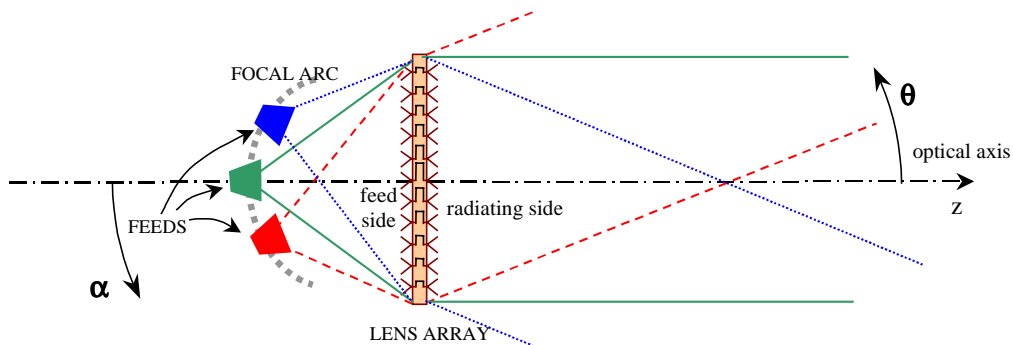
Fig. 1. Schematic of a planar discrete lens array with several independent feeds on its focal arc. Each feed controls a radiation pattern with the main beam pointing at a different angle off boresite.
